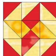
Swerende Ster
